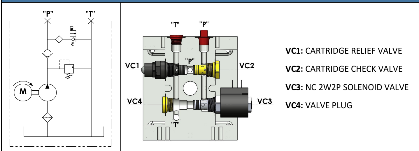
HYDRAULIC CIRCUIT 103
