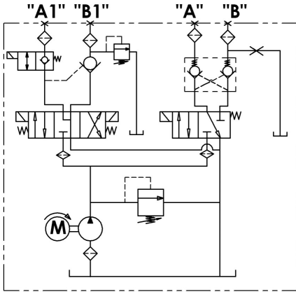
Hydraulic Circuit 217
