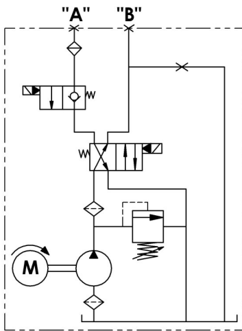
Hydraulic Circuit 109
