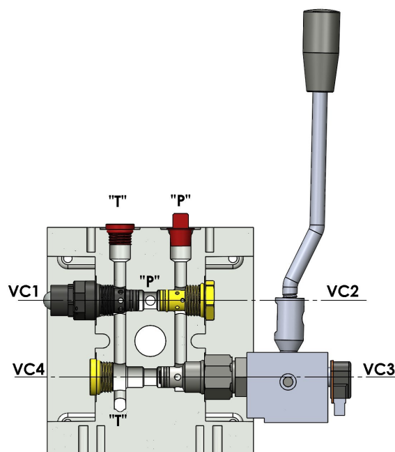
HYDRAULIC CIRCUIT 106
