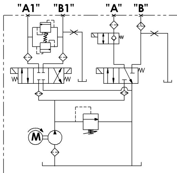
HYDRAULIC CIRCUIT 216
