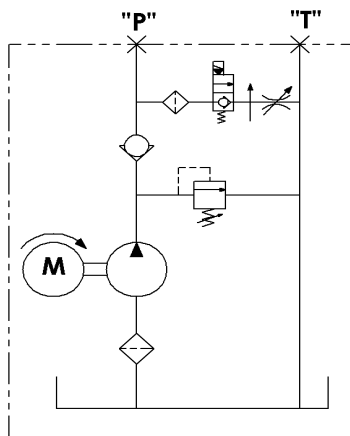
Hydraulic Circuit 104B
