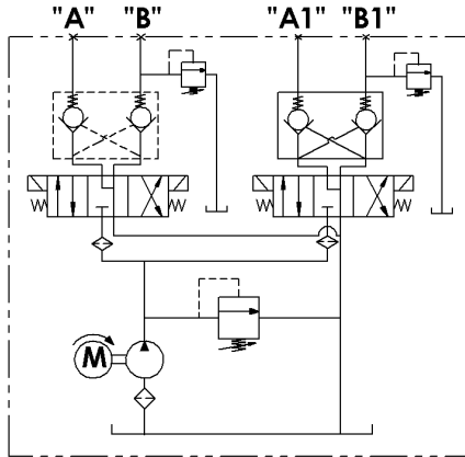
Hydraulic Circuit 208
