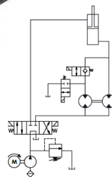
PRESSURE INTENSIFICATION CIRCUIT
