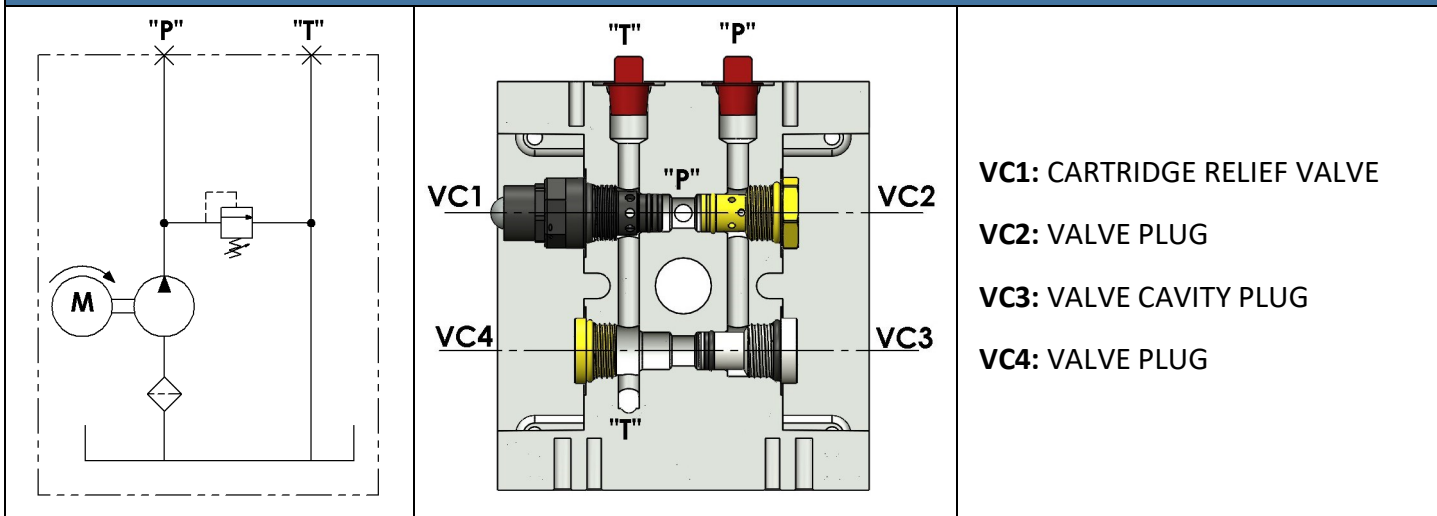
HYDRAULIC CIRCUIT 102B
