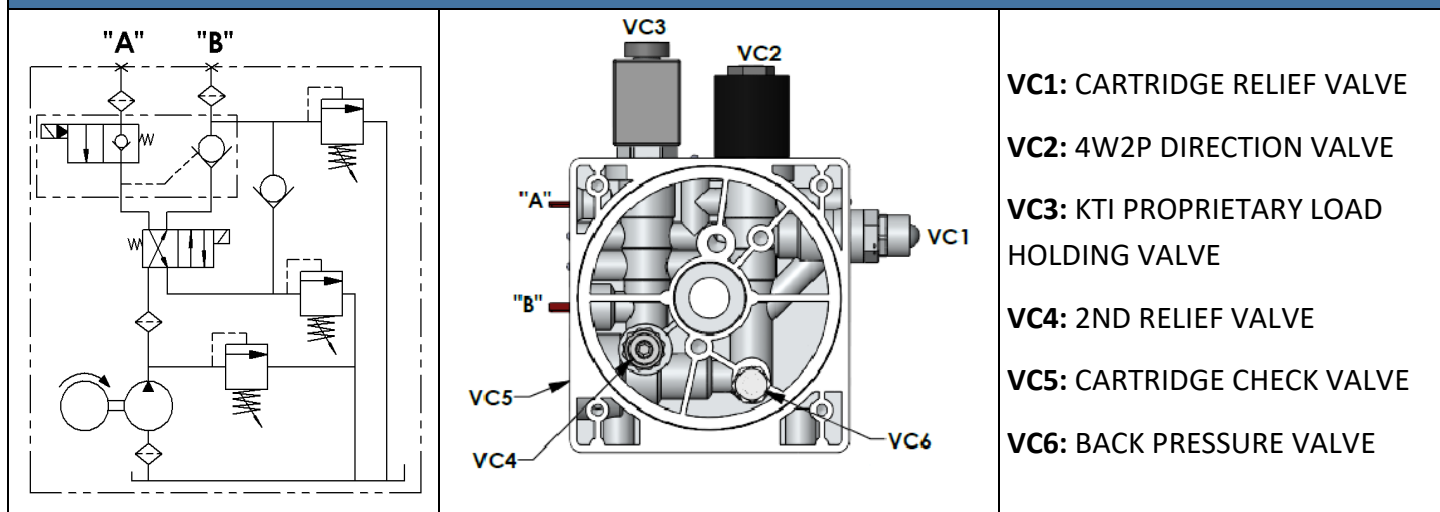
HYDRAULIC CIRCUIT 115*
