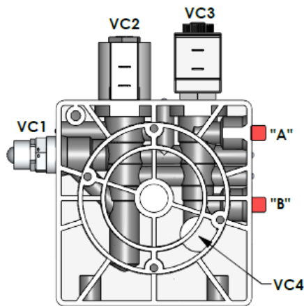
Hydraulic Circuit 109
