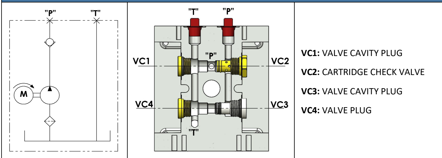
HYDRAULIC CIRCUIT 103
