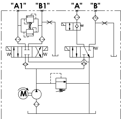
Hydraulic Circuit 216
